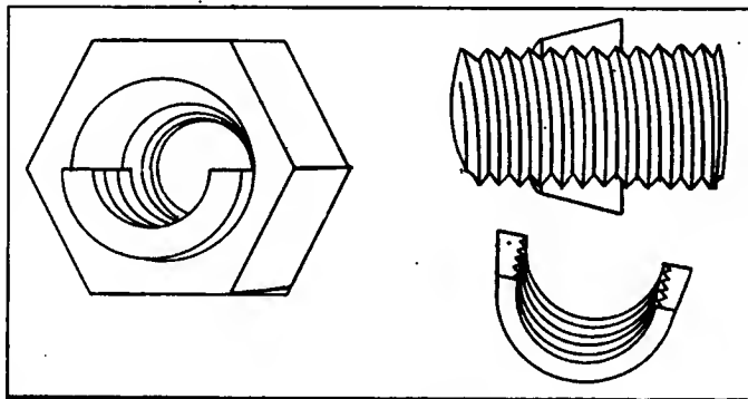
Fig. 1—Locknut for short bolt—a British improvement
